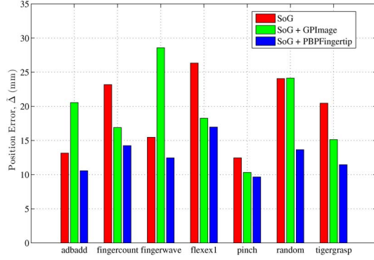
Figure 5. The average position error over the entire dataset for SoG only, SoG + GPIImage and SoG + PBPFingertips (ours).
