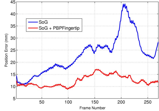
Figure 6. The average position error over the fingerwave dataset for SoG only and SoG + PBPFingertips (ours).
