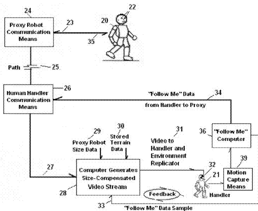
Figure 14B: Local Video Automatically Compensates for Proxy Size
