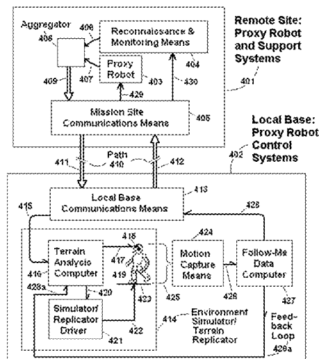
Diagram of Proxy Robotics Elements
